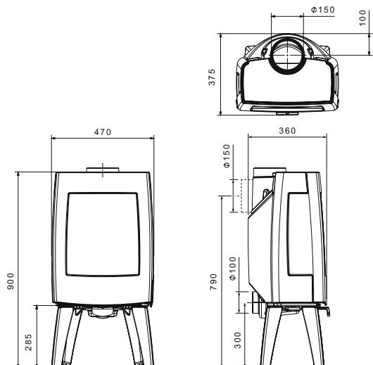
P20/21 | Sense 100 & 103 Wood Stoves
